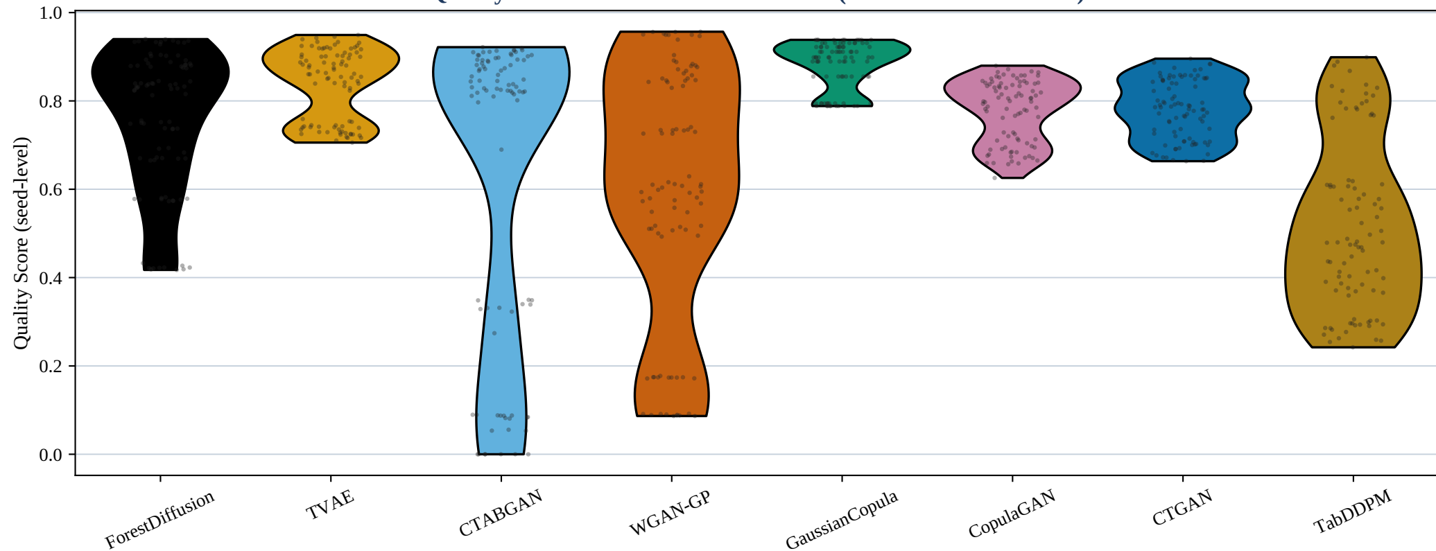
Quality Score — seed-level distribution (n = 10 seeds × datasets)
